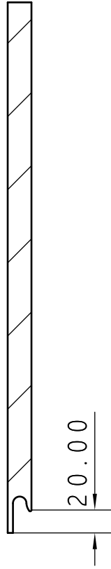
A - A (1:4)
